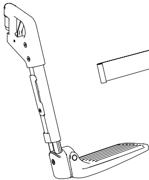
Legrest Standard
